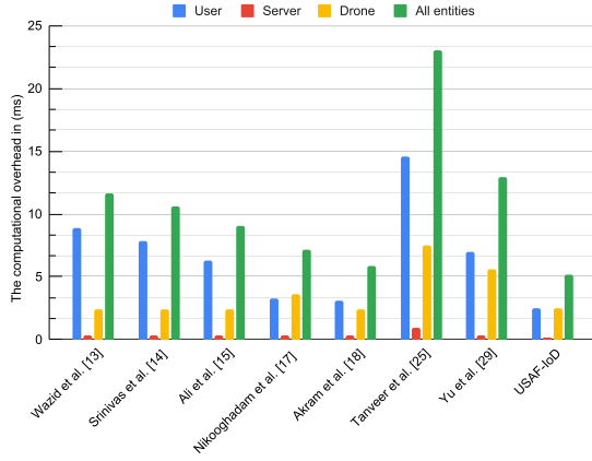
Fig. 4. Comparison of computation overhead.
