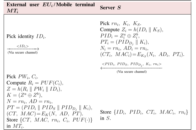
Fig. 2. Illustration of the user registration procedure.
