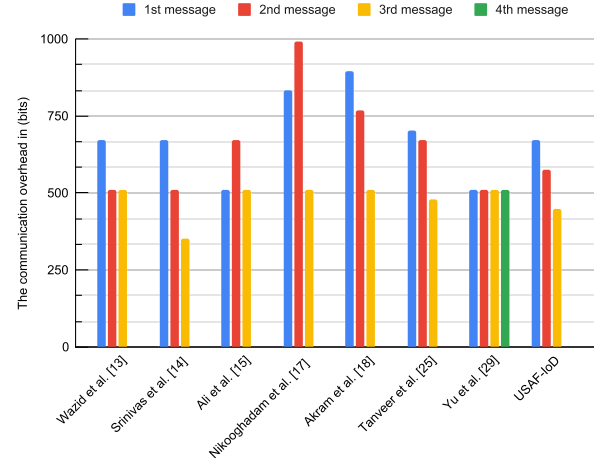
Fig. 5. Comparison of communication overhead.
