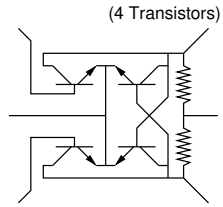
1961 Fairchild Bipolar RTL RS Flip-Flop
