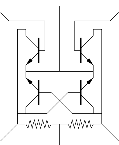
(4 Transistors)
