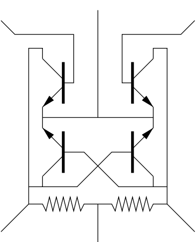
(4 Transistors)
