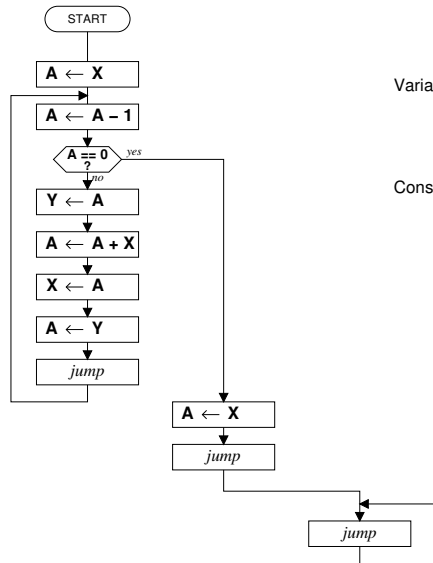
Simple Code for Example Processor
