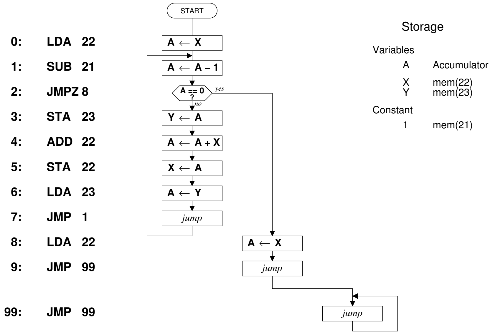
Simple Code for Example Processor
