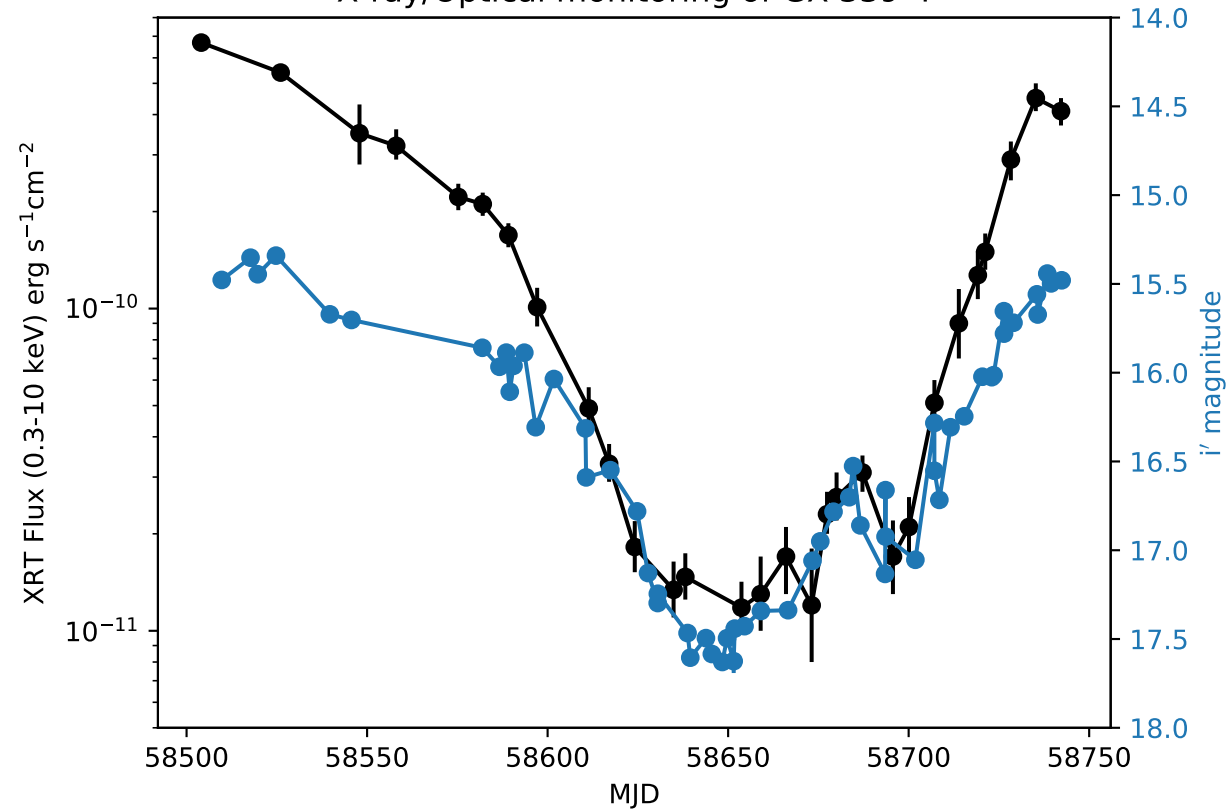
X-ray/Optical monitoring of GX 339-4
