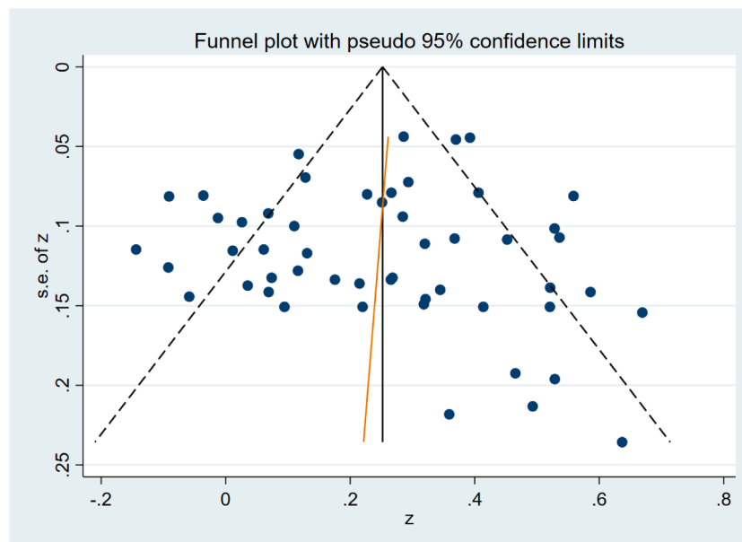
Fig. C.3. Funnel plot with z , reduced dataset (52 studies).
