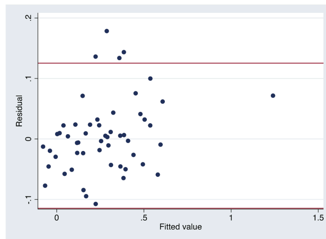
Fig. 5. Residual plot with z, complete dataset (53 studies).
