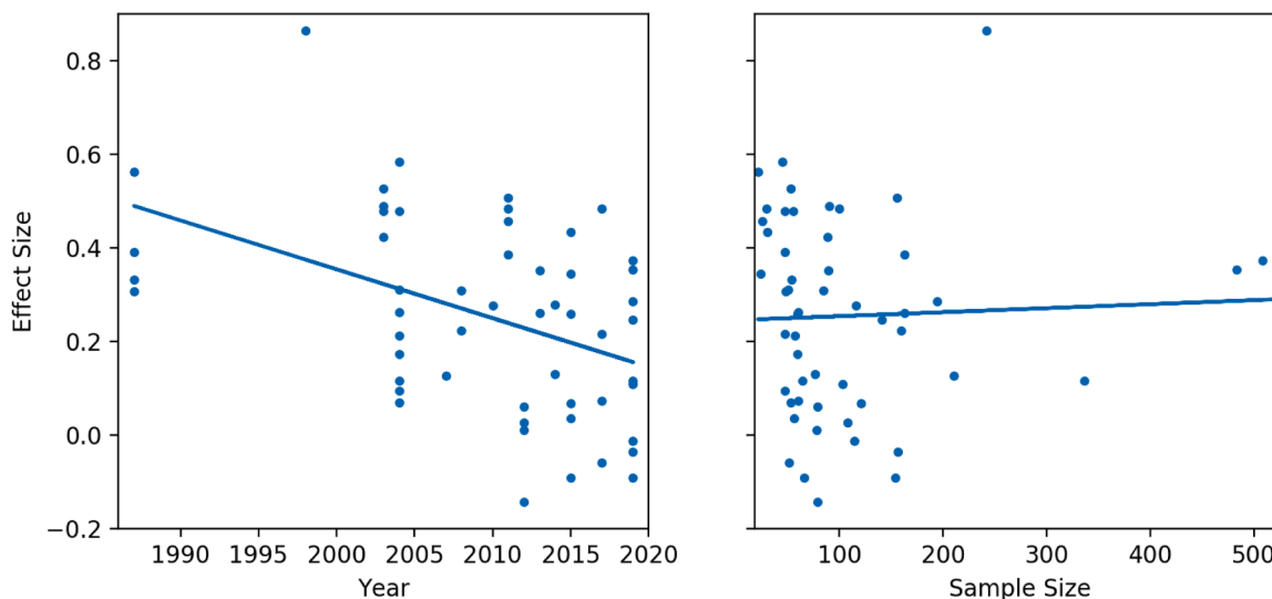
Fig. 3. Effect size as a function of publication year and sample size, complete dataset (53 studies).
