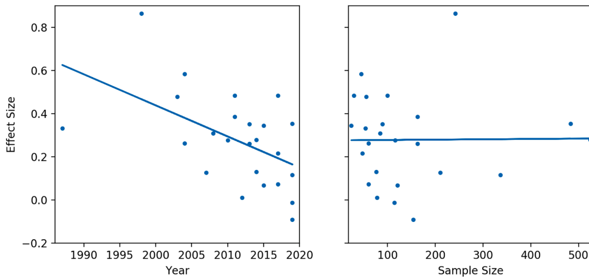
Fig. D.7. Effect size as a function of publication year and sample size, reduced dataset (24 studies).
