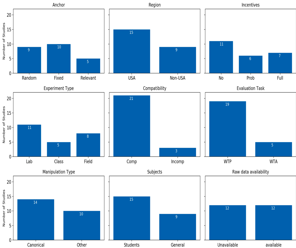
Fig. D.5. Summary of number of studies in each category, reduced dataset (24 studies).
